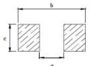
Recommend Land Pattern
