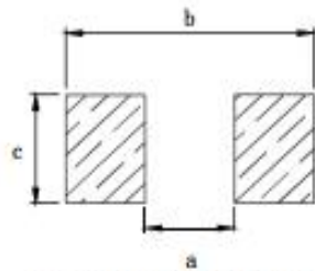
Recommend Land Pattern
