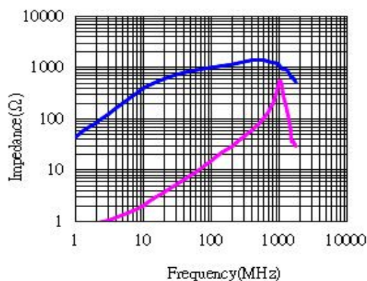
PERFORMANCE CURVES:
