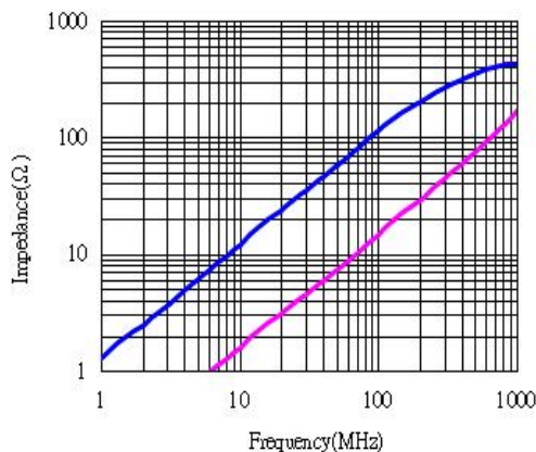
PERFORMANCE CURVES:
