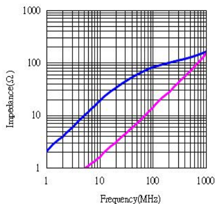
PERFORMANCE CURVES:
