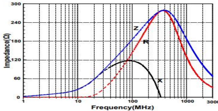
产品特性曲线图: Product Characteristic Curve
