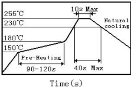
回流焊曲线 Reflow soldering profile
