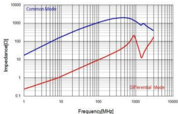
PERFORMANCE CURVES:
