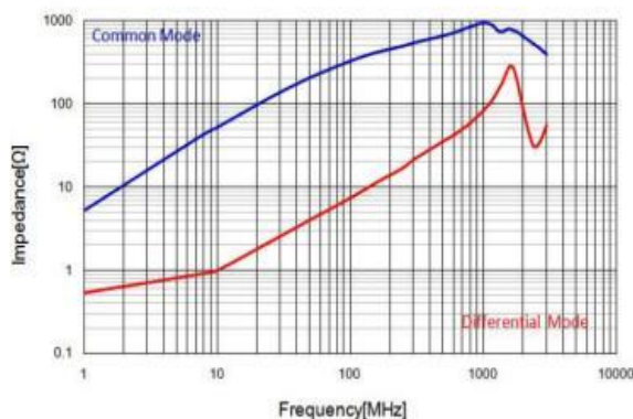
PERFORMANCE CURVES:
