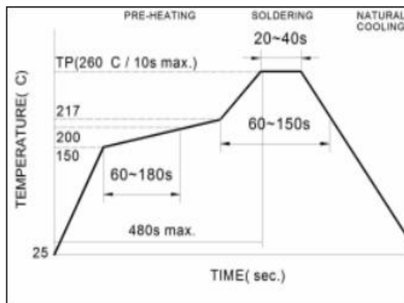
RECOMMENDED SOLDERING TEMP. GRAPH:
