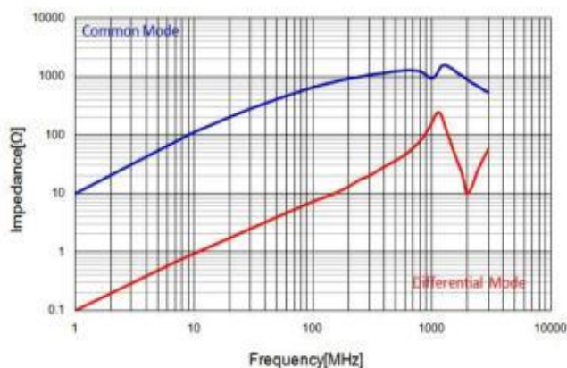
PERFORMANCE CURVES:
