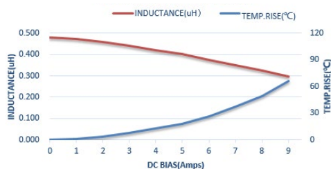
XRIM252010SR47MBCA
