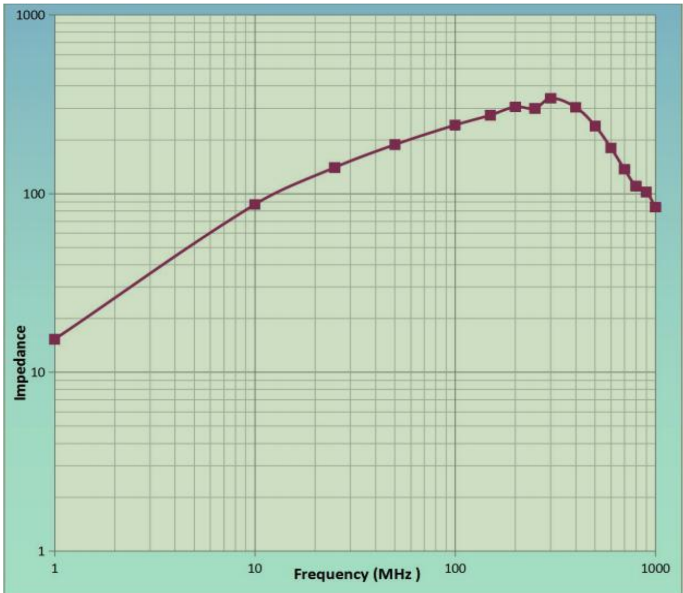
8 阻抗与频率的特性曲线 Characteristic curve of impedance and frequency
